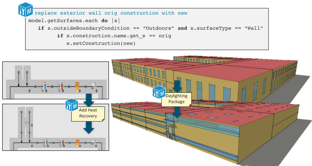
Figure II.2 Examples of OpenStudio measures
