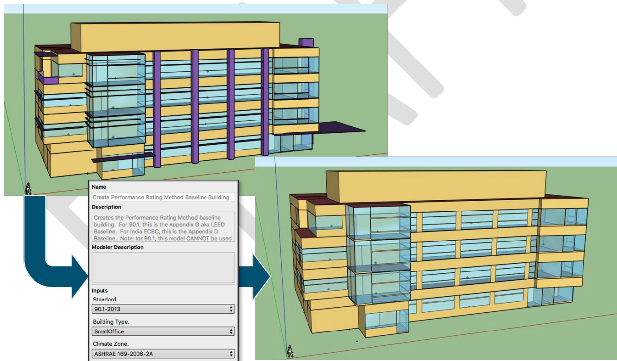
Figure II.3 The "create performance rating method baseline building" measure.
