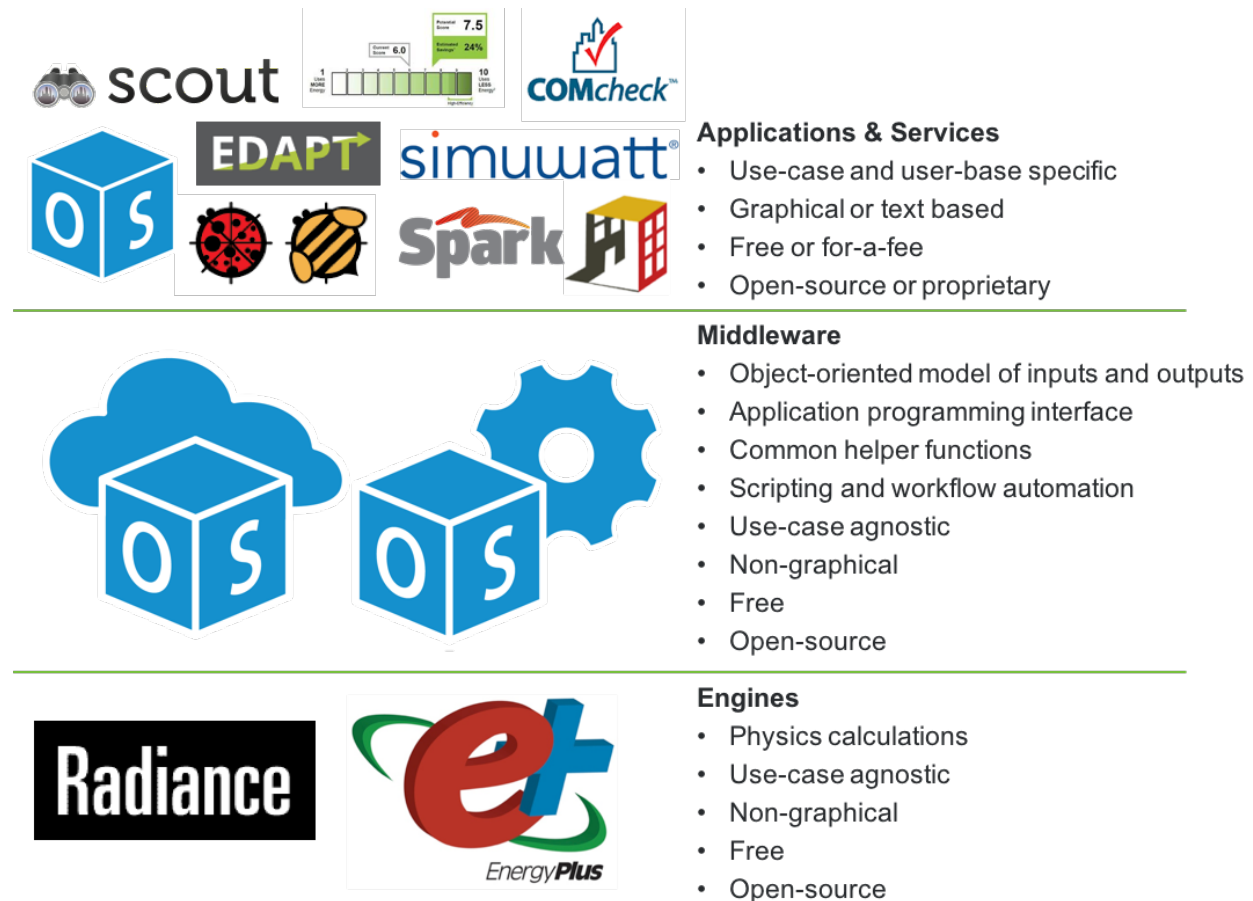
Figure II.1 BTO BEM software architecture and ecosystem.
