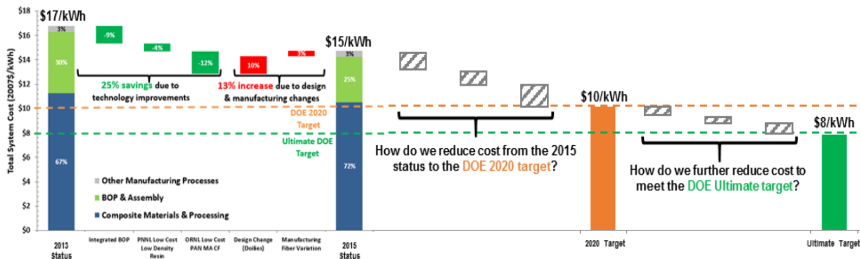
Figure 2: Waterfall plot of the 2013 700 bar compressed hydrogen storage system cost baseline and 2015 cost status update. The cost reductions identified from the 2013 baseline to the 2015 update are shown. Schematics of the 2020 target and Ultimate target are shown to illustrate DOE FCTO's request for input on how best to reach the targets.
