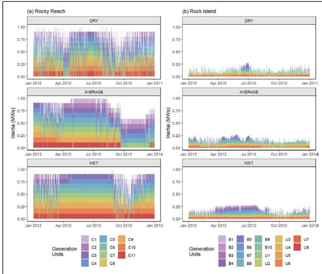
Figure 3. Hourly average inertia (MWs) contributed by all generating units for (a) Rocky Reach and (b) Rock Island run-of-river projects across dry, average, and wet years. Inertia response capabilities depend on water availability throughout the year, and the most generation during summer of wet years.
