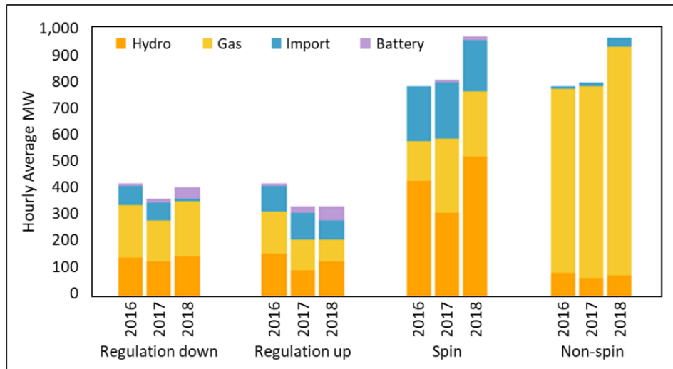
Figure 1. Hydropower contributions to essential reliability services in California Independent System Operator (CAISO). Relative to its share of generating capacity in CAISO, hydropower contributes a much larger share of regulation and spinning reserves.
