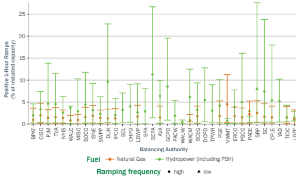
Figure 2. One-hour ramps per installed MW of hydropower and natural gas by balancing authority in 2019. Ramps by hydropower are often larger on average, at the hourly timescale, than natural gas plants.
