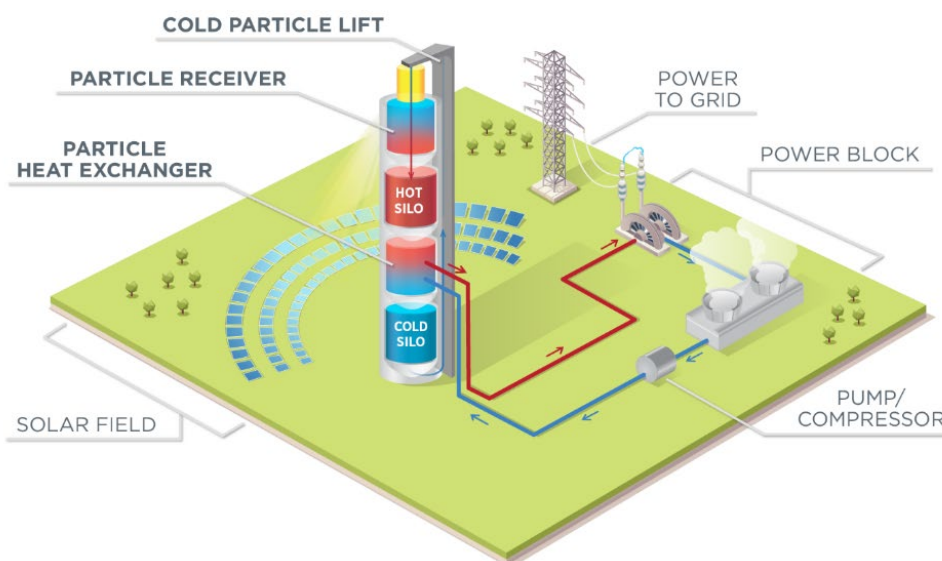
Figure 7. General design of a particle based CSP system; several forms of particle receiver shape, design and layout of silos, heat exchanger and intermediate lift are feasible; power block is a representation
