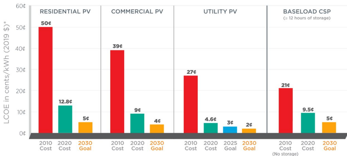
Figure 2: Cost of energy for PV and CSP technologies
