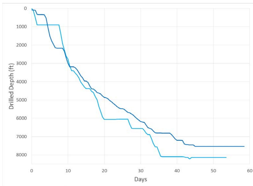
Figure 2: Depth vs Days for drilling of FORGE wells
