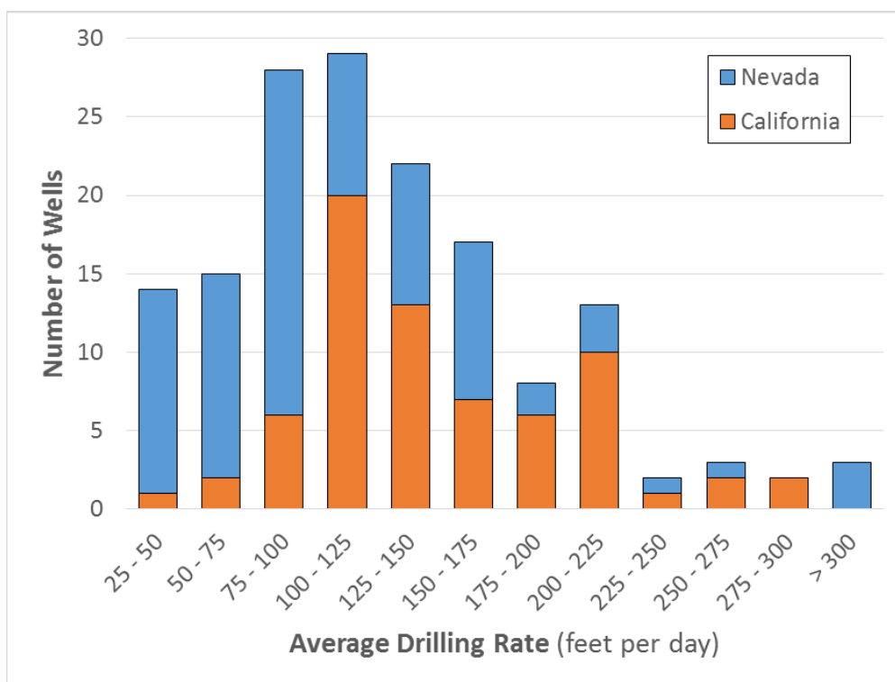
Figure 1: Rate of Drilling for Domestic Geothermal Injection/Production Wells Drilled for California and Nevada (2005-2010). Note that these data do not include pre-spud engineering time; days for each well were determined from Spud date to Completion date as reported to the states.
