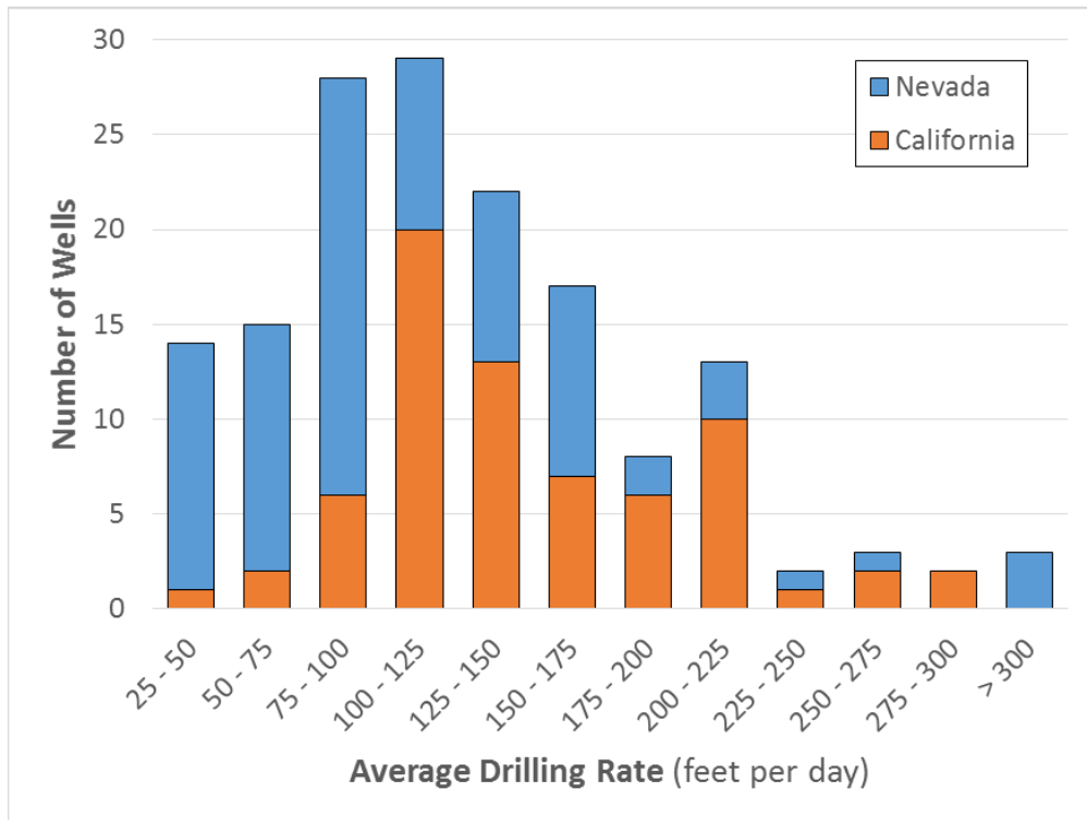
Figure 1: Rate of Drilling for Domestic Geothermal Injection/Production Wells Drilled for California and Nevada (2005-2010). Note that these data do not include pre-spud engineering time; days for each well were determined from Spud date to Completion date as reported to the states.
